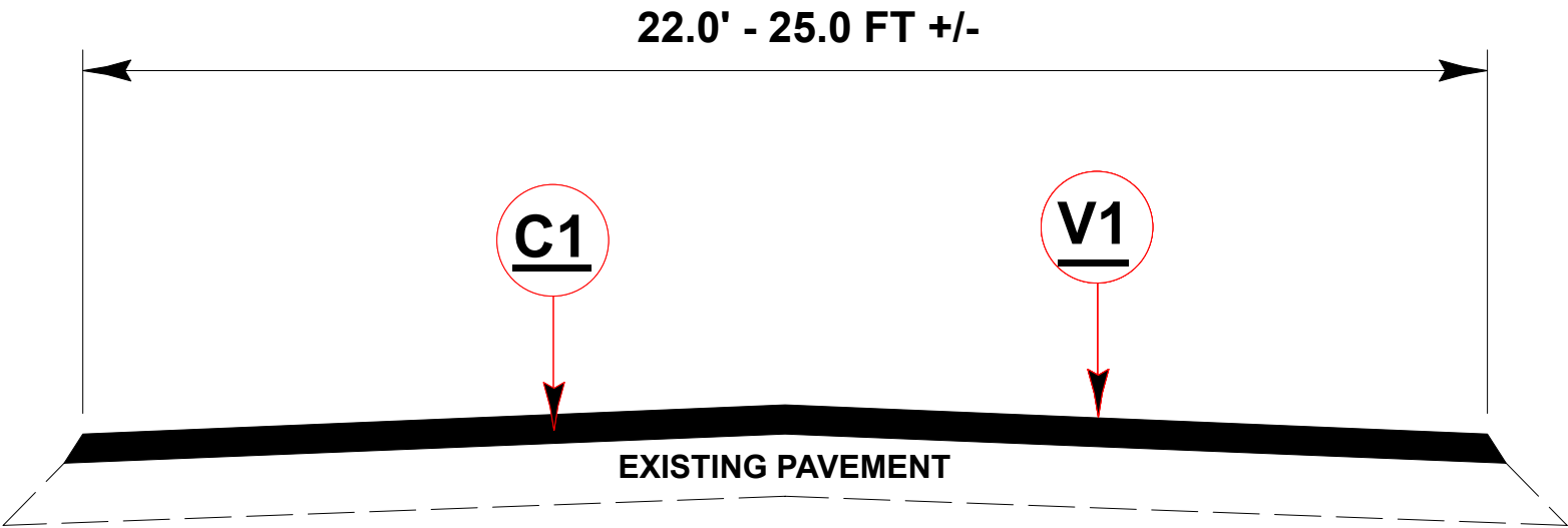
TYPICAL SECTION # 5 MAP(S) # 12 & 19
